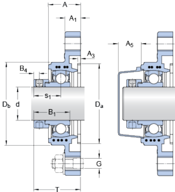
FYTBK 20 FE Bearing 2D drawings and 3D CAD models
